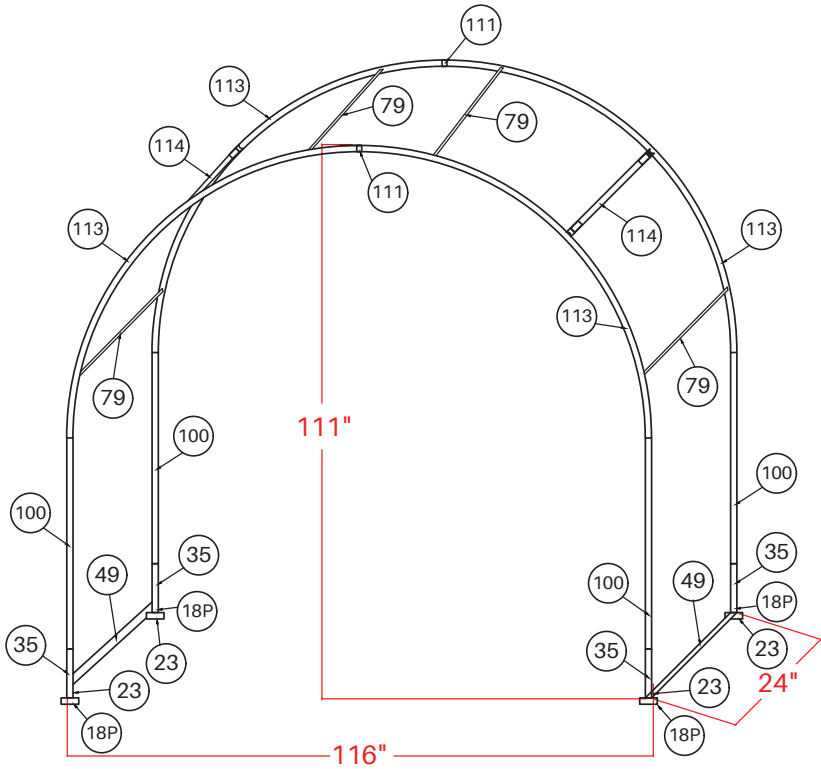
Straight Poles
